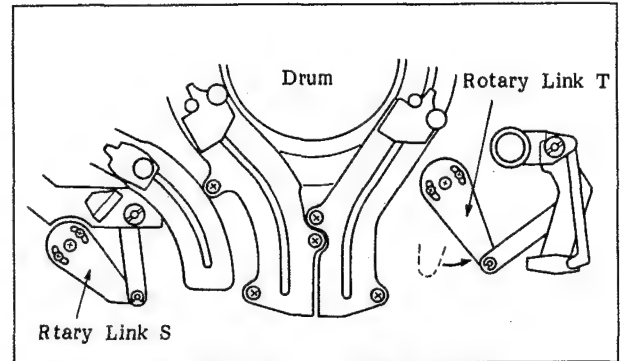
Fig. 6-65. Replacement of Link Wheels S/T
